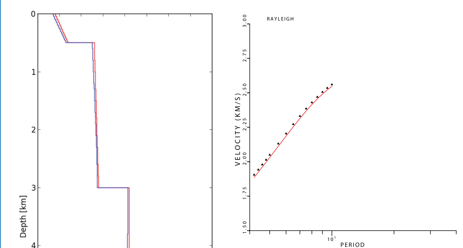
The longer periods also recover the true structure very well. The differences between the inverted model and the true structure are a bit larger than for the shorter periods, however.
