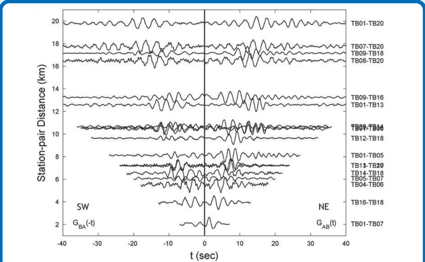
Huang et al. (2010) obtain Green's functions by crosscorrelating ambient noise recorded between 0.5 and 3 seconds period. These can be used to determine surface wave dispersion curves.
