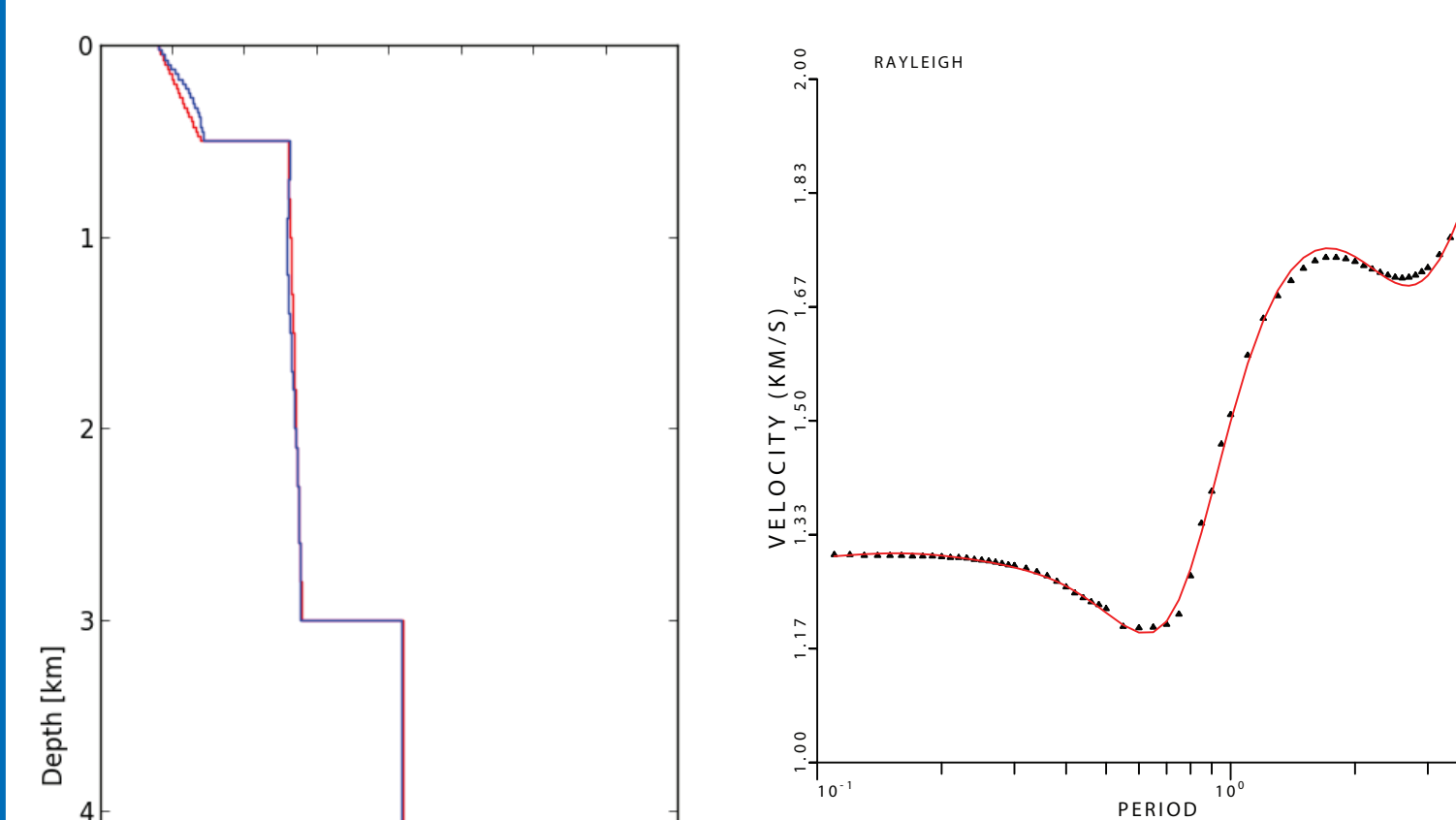
We first invert the measured dispersion curve using the same model used to calculate the synthetic waveforms as a starting model. Not surprisingly the true structure is well recovered by the inversion.
