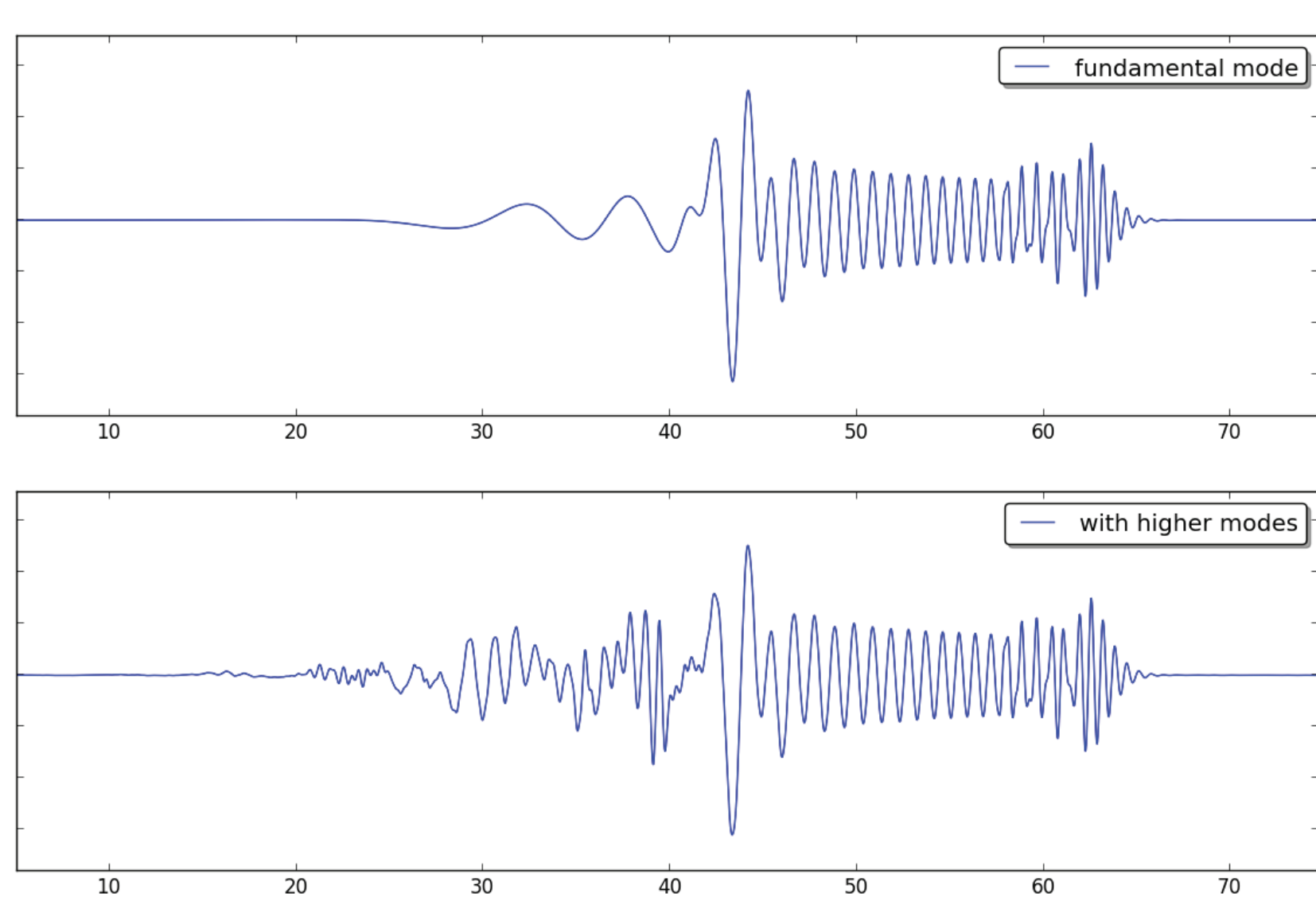
However, a comparison of just the fundamental mode with the first 30 modes (including the fundamental) reveals that major differences exist only for the body waves arriving earlier. The surface waves are near identical so we proceed by using just the fundamental mode
