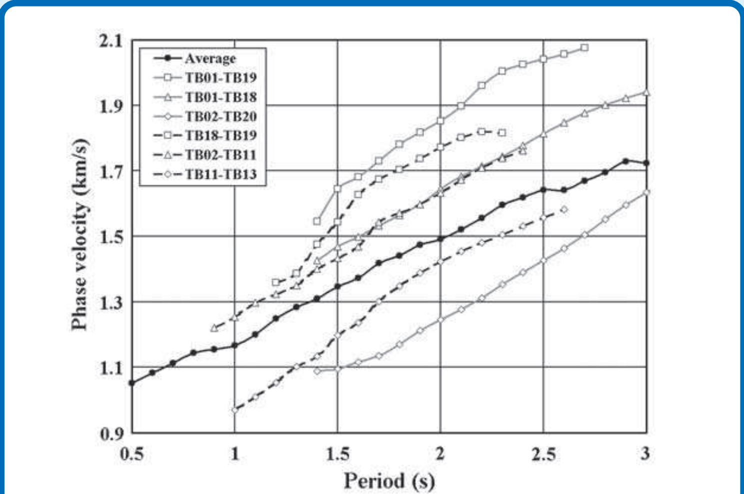
Analysing the the Green's functions yields phase velocity dispersion curves, which in turn provide insights into the crustal structure between two stations (Huang et al., 2010).
