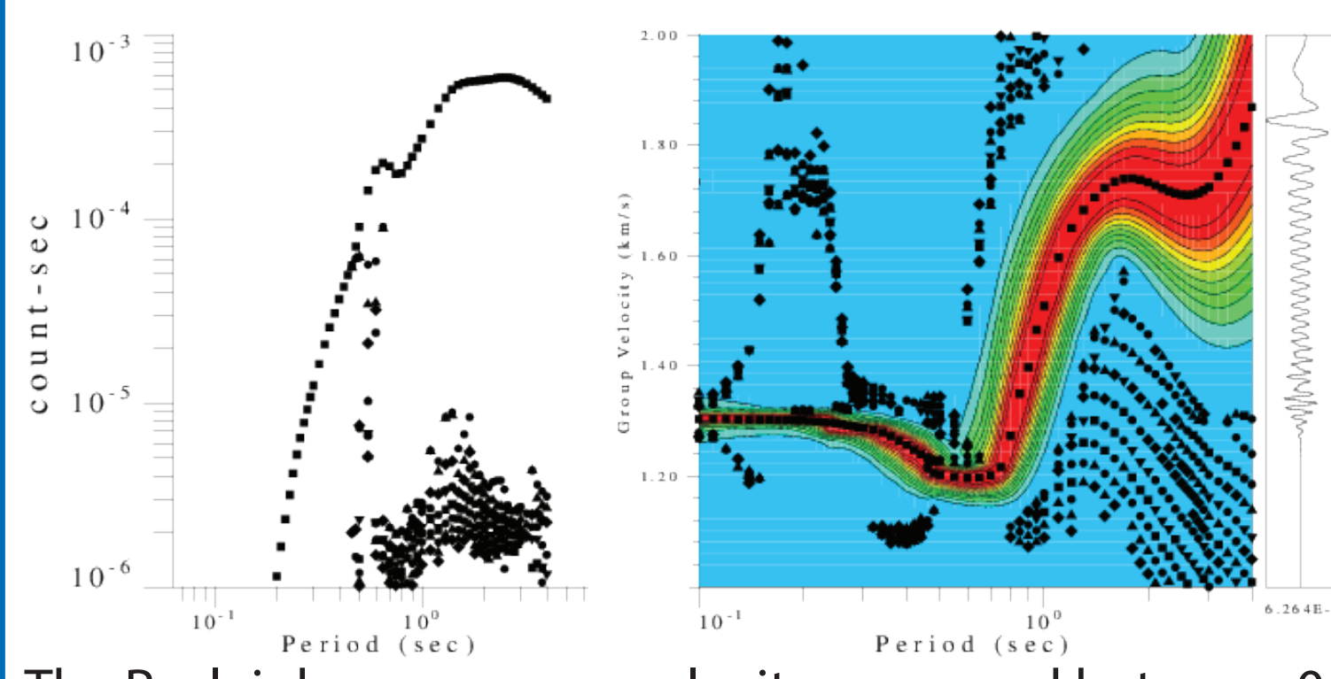
The Rayleigh wave group velocity measured between 0.1 and 4 seconds is relatively complex; the dispersion curve reveals two Airy phases (slope = 0). However, the curve itself is easily measured.
