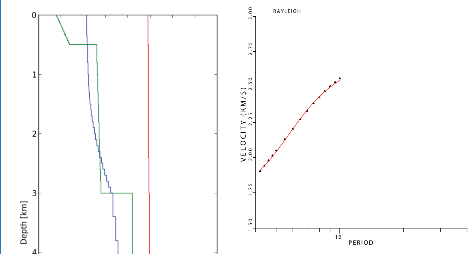
At a first glance the recovered model looks similar to the one obtained at shorter periods. However the inversion does not yield the shallow low velocities.
