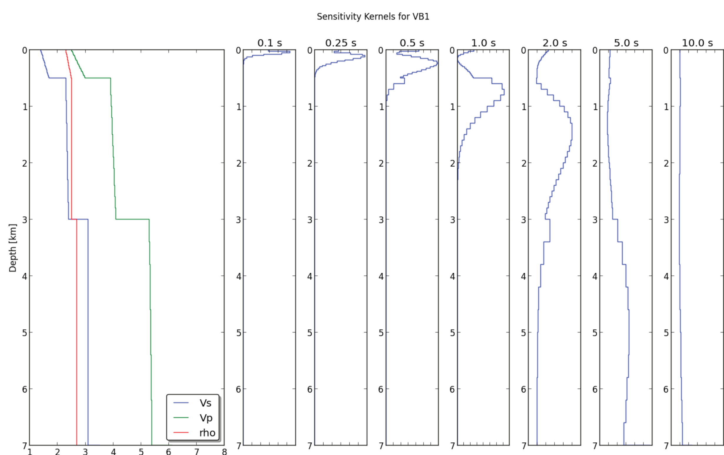
We calculate fundamental mode Rayleigh wave phase velocity sensitivities to illustrate the dependence of measured phase velocities to S-velocities at depth. At short periods (0.1 to 1 second) phase velocity depends only on the top few hundred meters. For longer periods the phase velocity rapidly becomes more sensitive to the S-velocities of the mid- to lower crust. Therefore we must use the short periods if we want to investigate the velocity structure of the uppermost crust.
