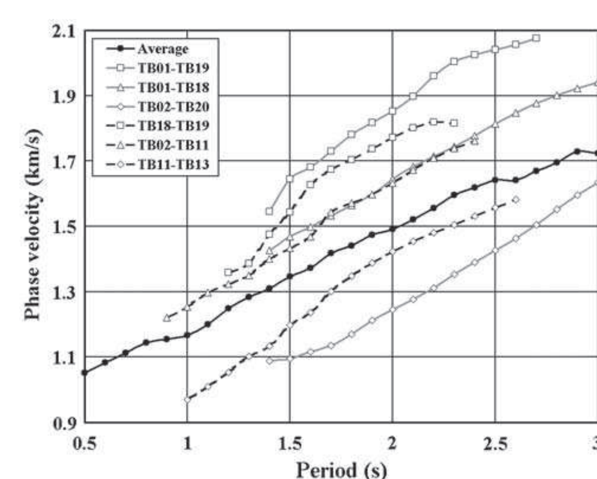
Analysing the the Green's functions yields phase velocity dispersion curves, which in turn provide insights into the crustal structure between two stations (Huang et al., 2010).
