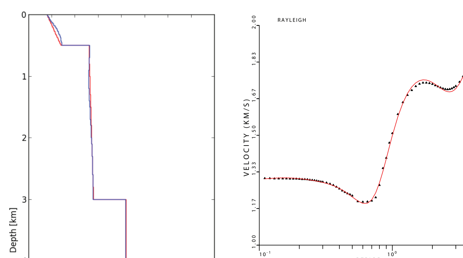
We first invert the measured dispersion curve using the same model used to calculate the synthetic waveforms as a starting model. Not surprisingly the true structure is well recovered by the inversion.
