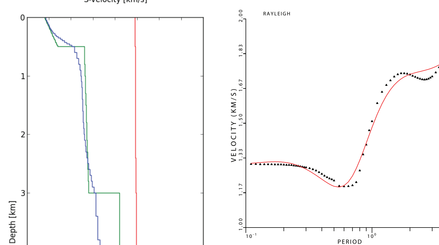
Using a simple starting model with a constant velocity in the upper crust the true structure is not recovered as well. Importantly though, the slow velocities in the uppermost layers are seen in the inverted model.
