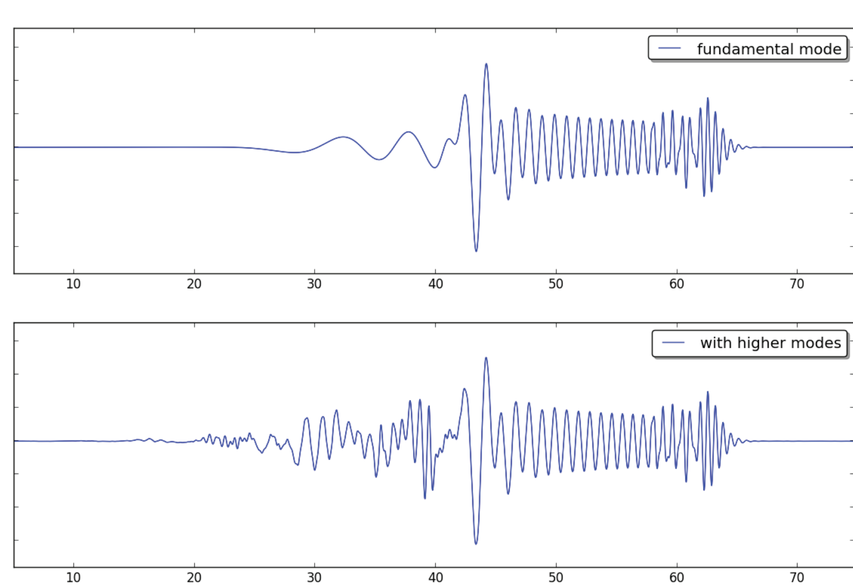
The sources of ambient noise recorded by seismometers are most likely generated at the surface. Hence we calculate synthetic seismograms assuming a vertical force acting on the free surface, recorded on the vertical component of seismic station at a distance of 75 km. The full waveform is obtained by model summation.
