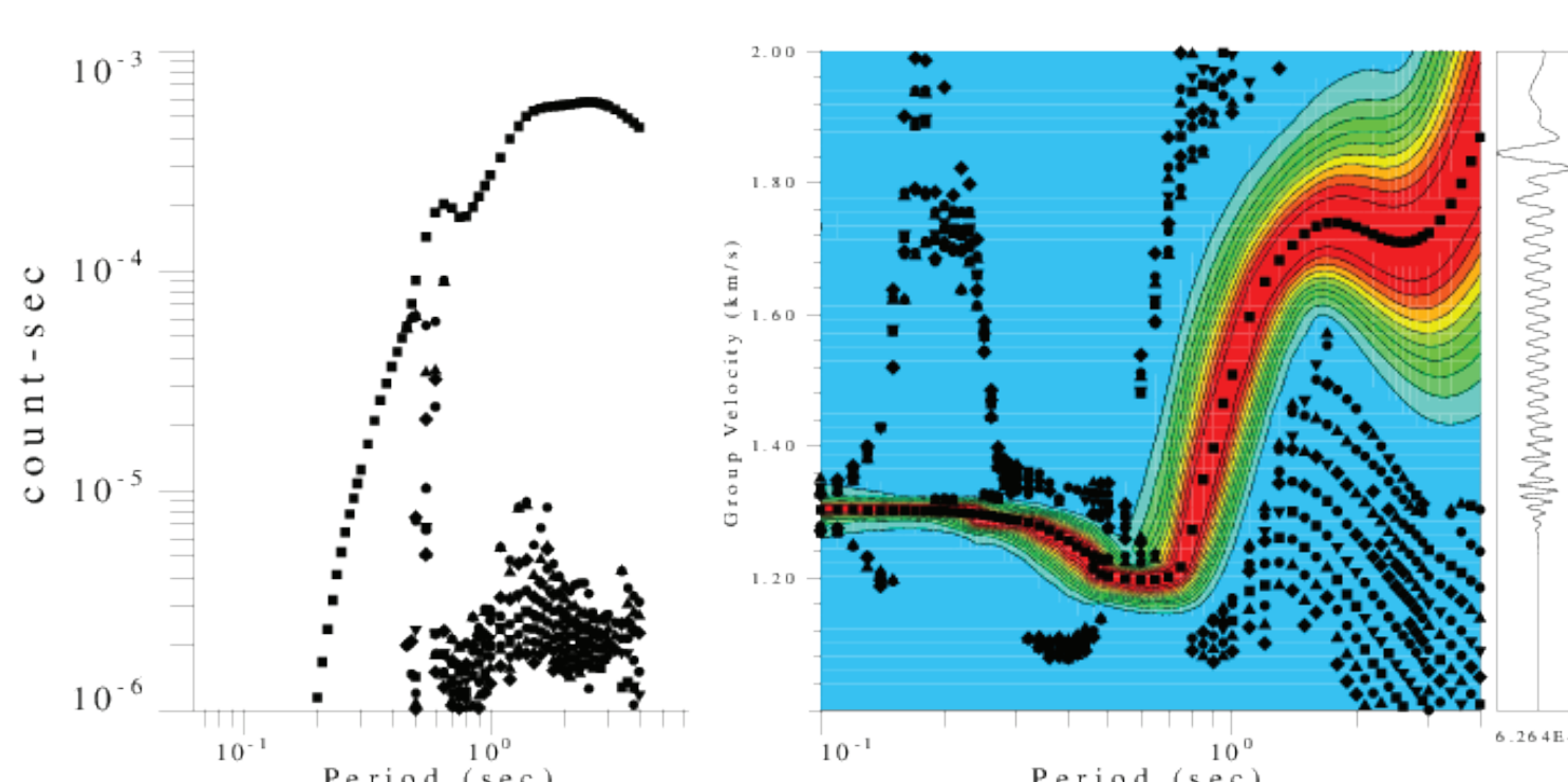
The Rayleigh wave group velocity measured between 0.1 and 4 seconds is relatively complex; the dispersion curve reveals two Airy phases (slope = 0). However, the curve itself is easily measured.
