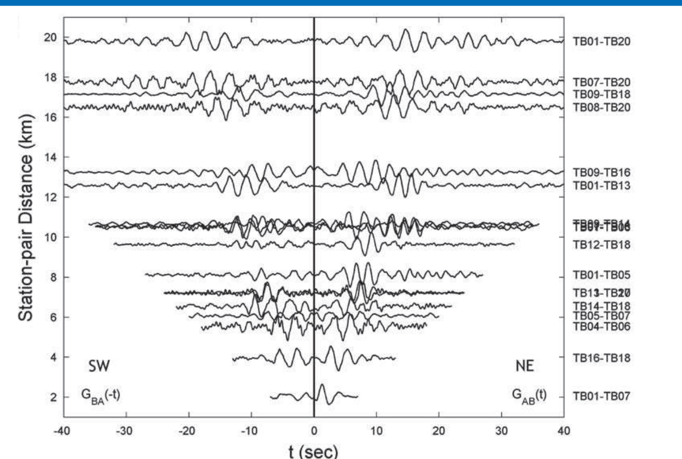
Huang et al. (2010) obtain Green's functions by crosscorrelating ambient noise recorded between 0.5 and 3 seconds period. These can be used to determine surface wave dispersion curves.
