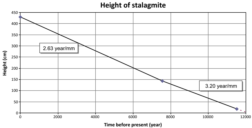
Fig. 12 The height of the stalagmite we investigated as a function of time going back into the past calculated by the results of the age dating. The numbers in the boxes show the mean growth rate at two parts of the stalagmite
