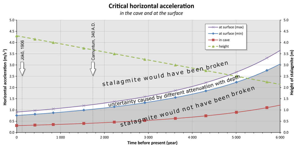
Fig. 14 Constraints on critical horizontal ground acceleration (CHGA) at the surface and in the cave provided by the height of the IVSTM, which is still intact and provided by the depth of the
